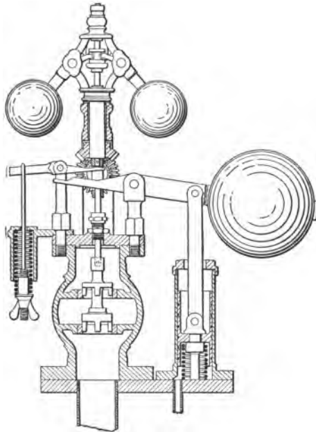
FIG. 81.—Clayton governor.
